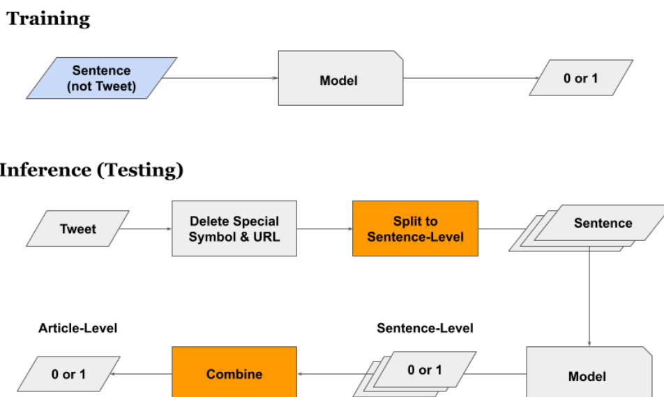
Figure 5.7: Pipeline for dealing with improper task definition. The Model mentioned here can refer to the Model in Figure 3.1.
