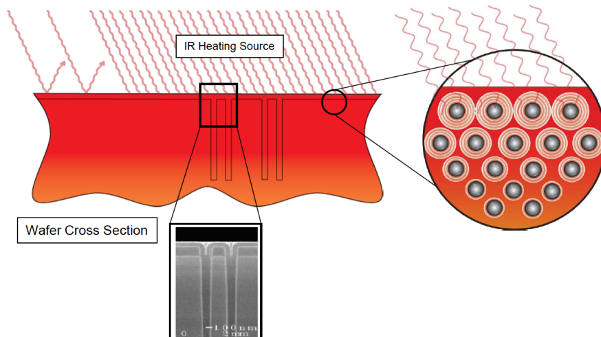
Figure 5.5 RTA heating, heating is limited by thermal diffusivity and surface temperature.
