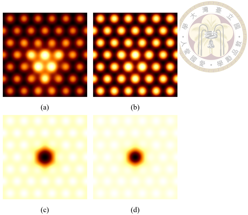
Figure 3.5: Comparison of simulations using different tungsten diselenide models. Initial z position is 0.5nm and lateral dimensions are 2 \times 2 nm. (a) Single-orbital model with a tungsten vacancy. (b) Multi-orbital model with a tungsten vacancy. (c) Single-orbital model with a (top) selenide vacancy. (d) Multi-orbital model with a (top) selenide vacancy.
