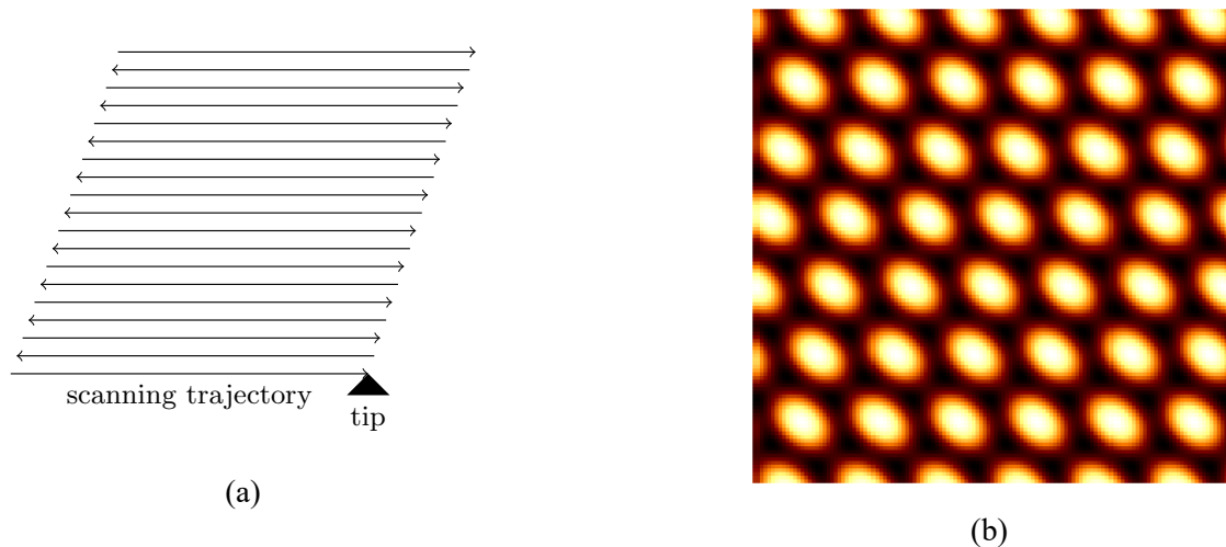
Figure 1.6: Illustration of the thermal drift effect in the fast scanning axis. (a) Scanning trajectory of the STM tip. (b) Resulting image.
