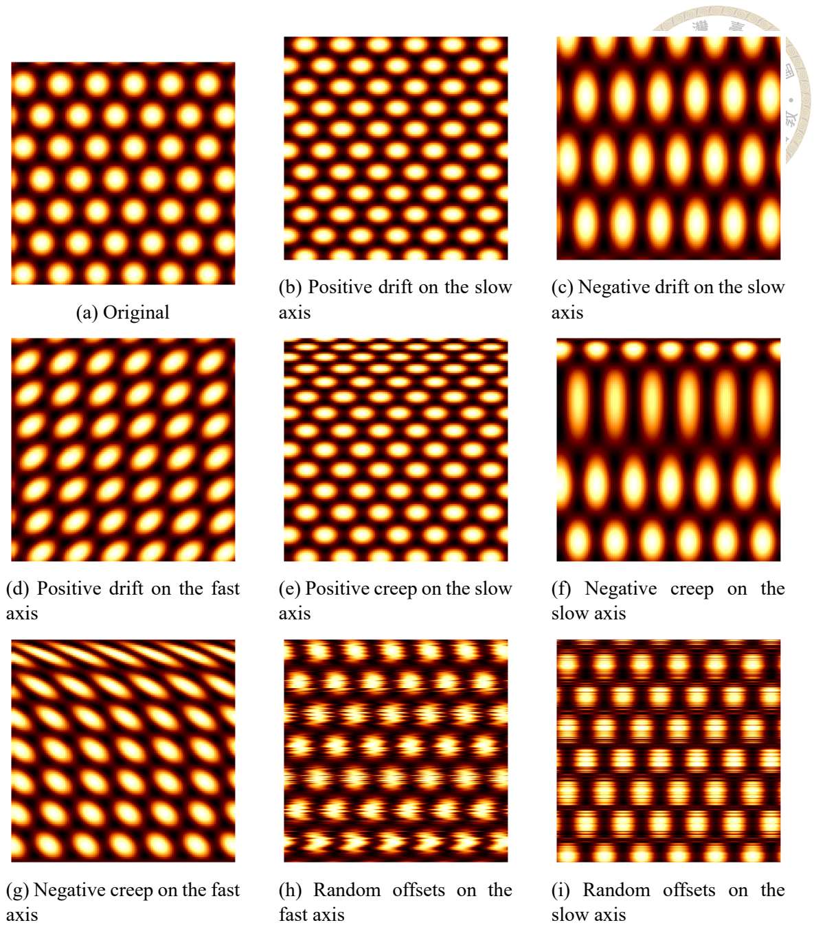
Figure 2.1: Types of lateral scanning distortions.
