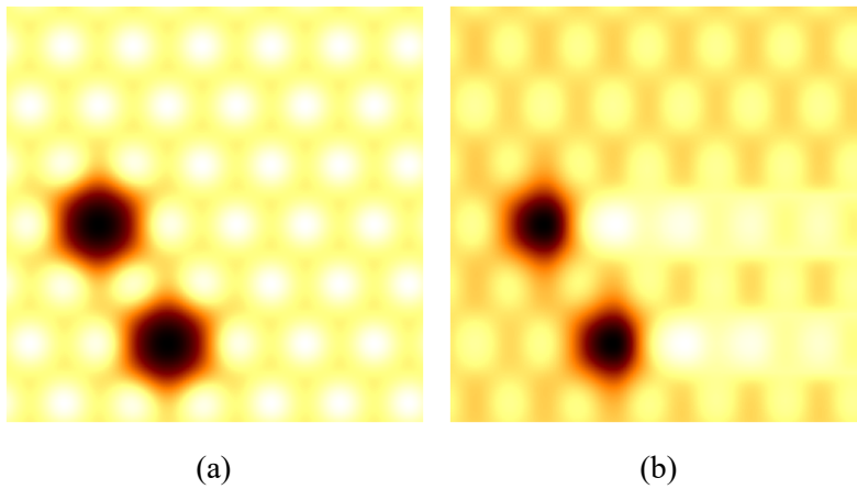
Figure 2.3: Effect of hysteresis on a defective lattice. (a) No hysteresis. (b) With hysteresis, showing characteristic trailing artifacts.
