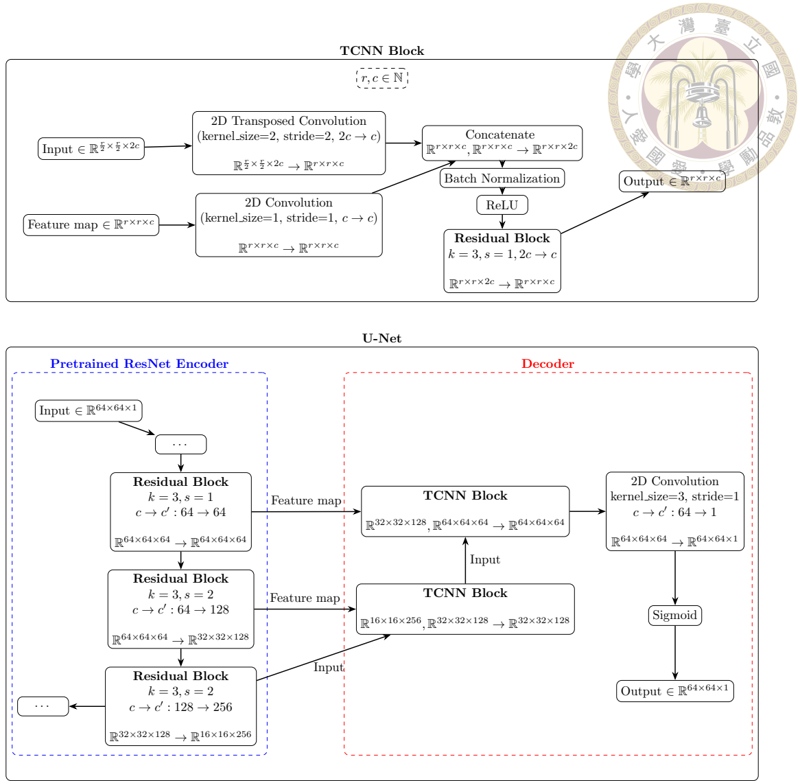
Figure 3.13: Modified U-Net structure and its components.
