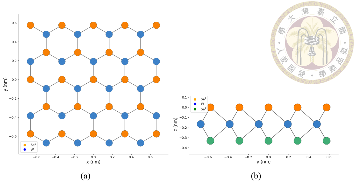
Figure 3.1: WSe 2 lattice. (a) Top-down view. (b) Side view.
