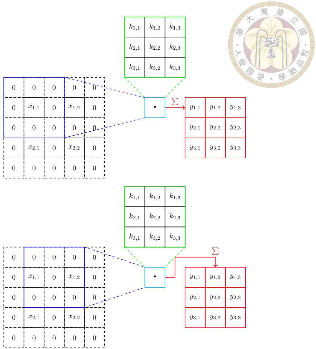
Figure 1.9: Illustration of a transposed convolution with a stride of two pixels.
