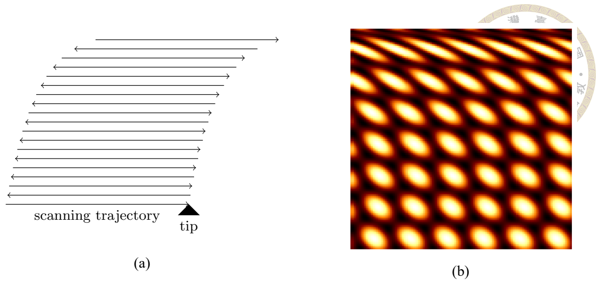
Figure 1.5: Creep effect in the fast scanning axis. (a) Scanning trajectory of the STM tip. (b) Resulting image.
