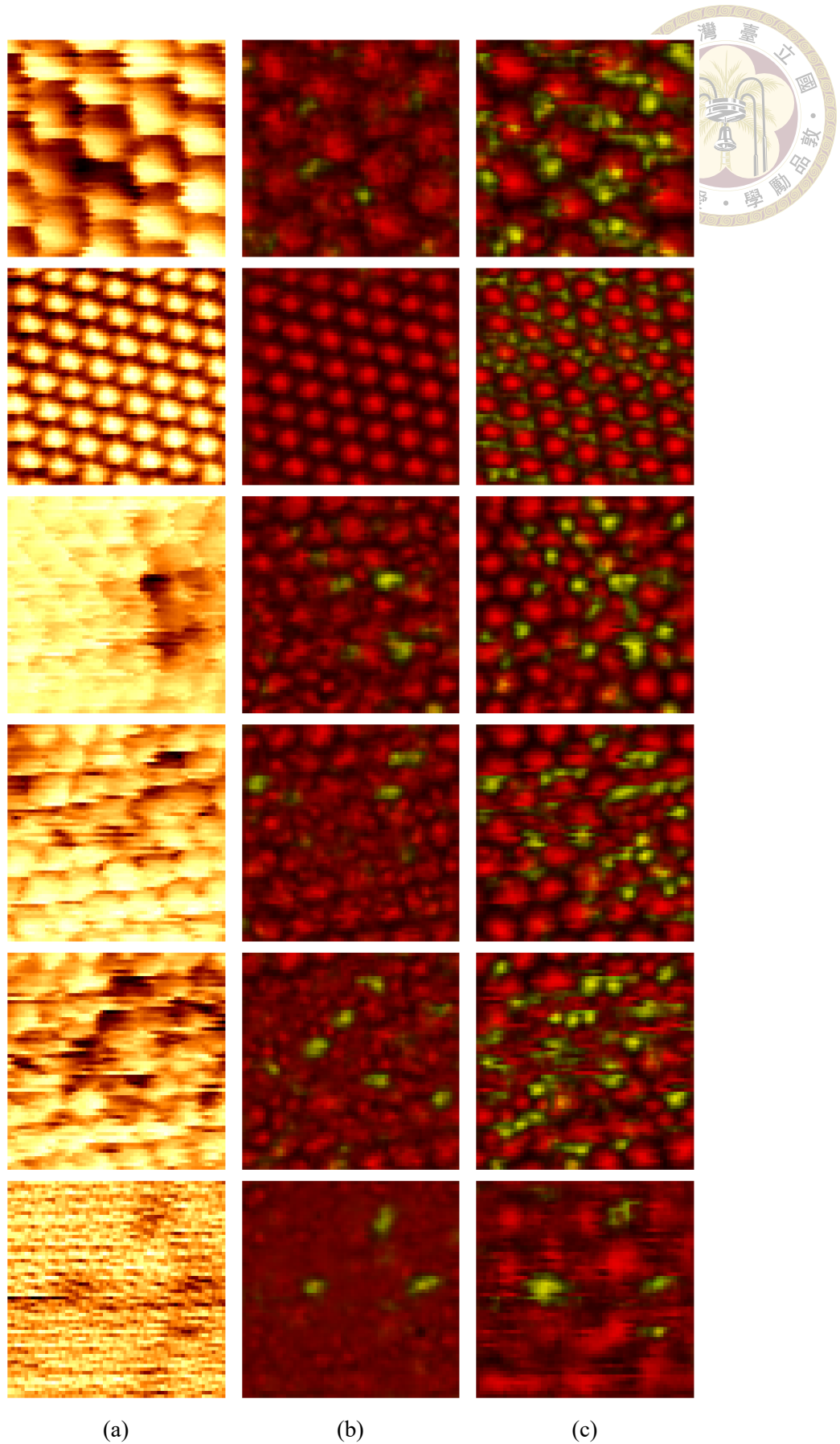
Figure 3.16: Testing of U-Net defect localization model on real samples. No ground truth available. (a) Input image. (b) Prediction by U-Net trained using the main dataset including the full PID simulation. (c) Prediction by U-Net trained using the control dataset without PID simulation.
