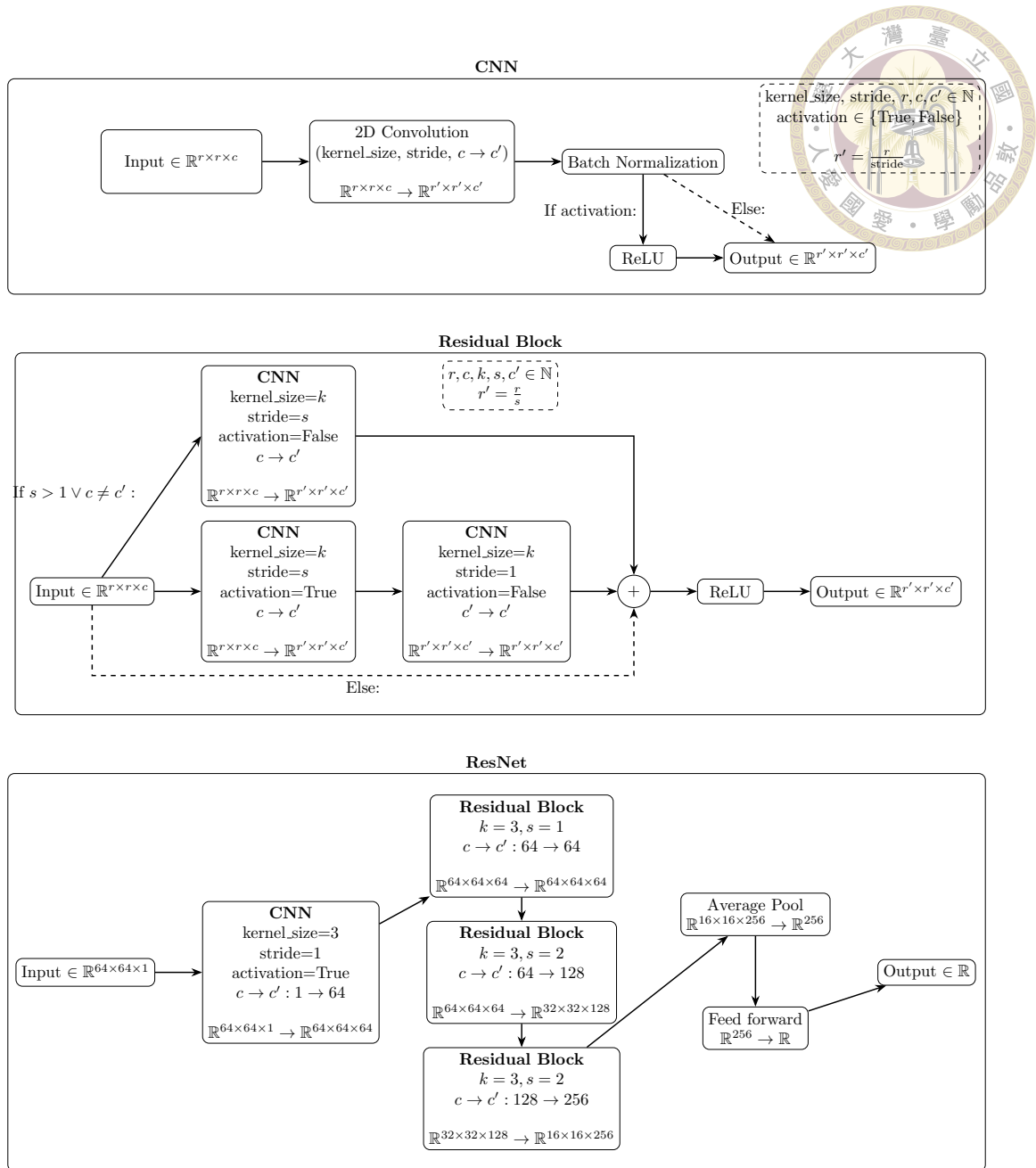
Figure 3.12: Modified ResNet structure and its components.
