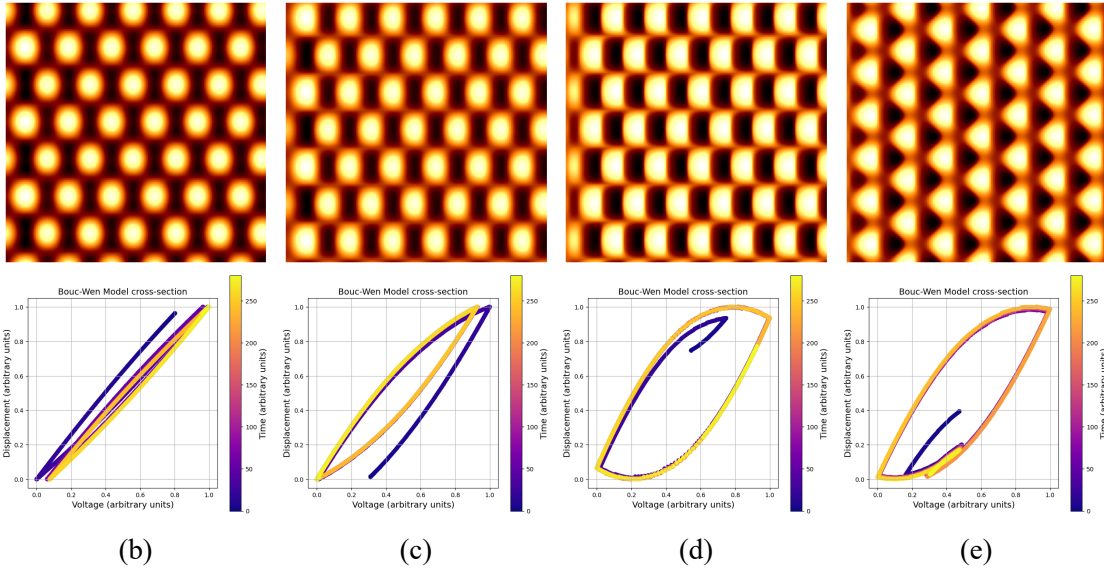
Figure 2.2: Hysteresis effect on a non-defective lattice. Hysteresis parameters \beta = 0.6, \gamma = 0.6 are common. (a) No hysteresis: A = 0 , (b) Moderate hysteresis: A = 0.4 , (c) Strong hysteresis: A = 0.7 , (d) Very strong hysteresis: A = 0.9 . (e) Very strong hysteresis, sample rotated by 30^\circ .
