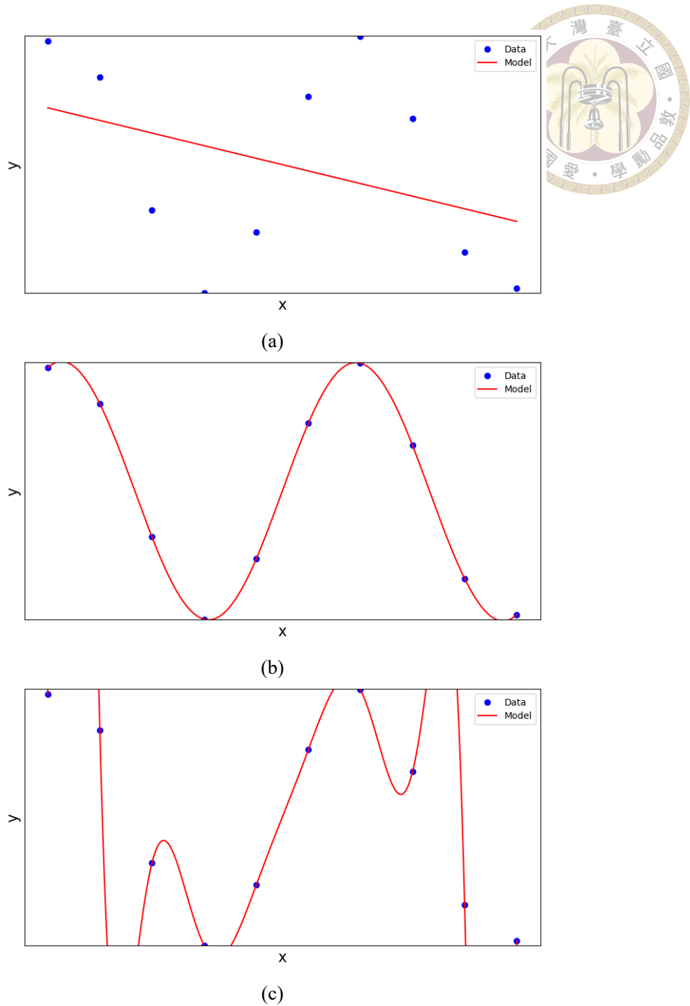
Figure 1.7: Illustration of underfitting (a), appropriate capacity (b) and overfitting (c).
