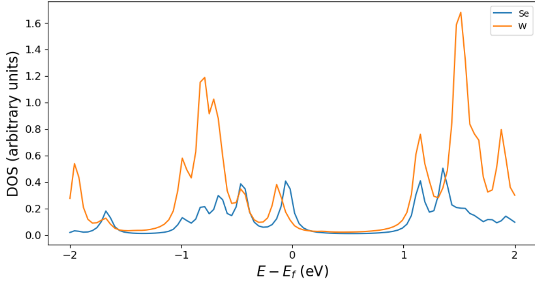
Figure 3.2: Simulated density of states for tungsten and selenide atoms in monolayer WSe 2 .
