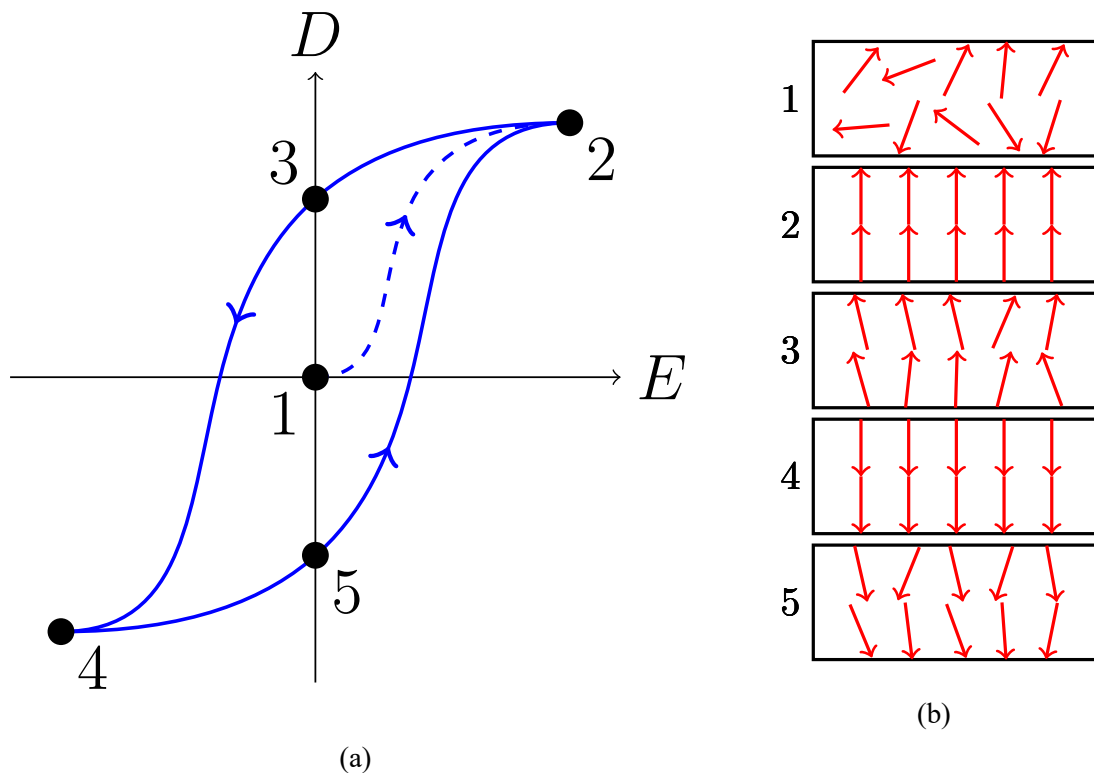
Figure 1.4: Illustration of the domain orientation on the applied electric field. (a) Electric displacement field change ( D = \epsilon_0 E + P ). (b) Domain reorientation.
