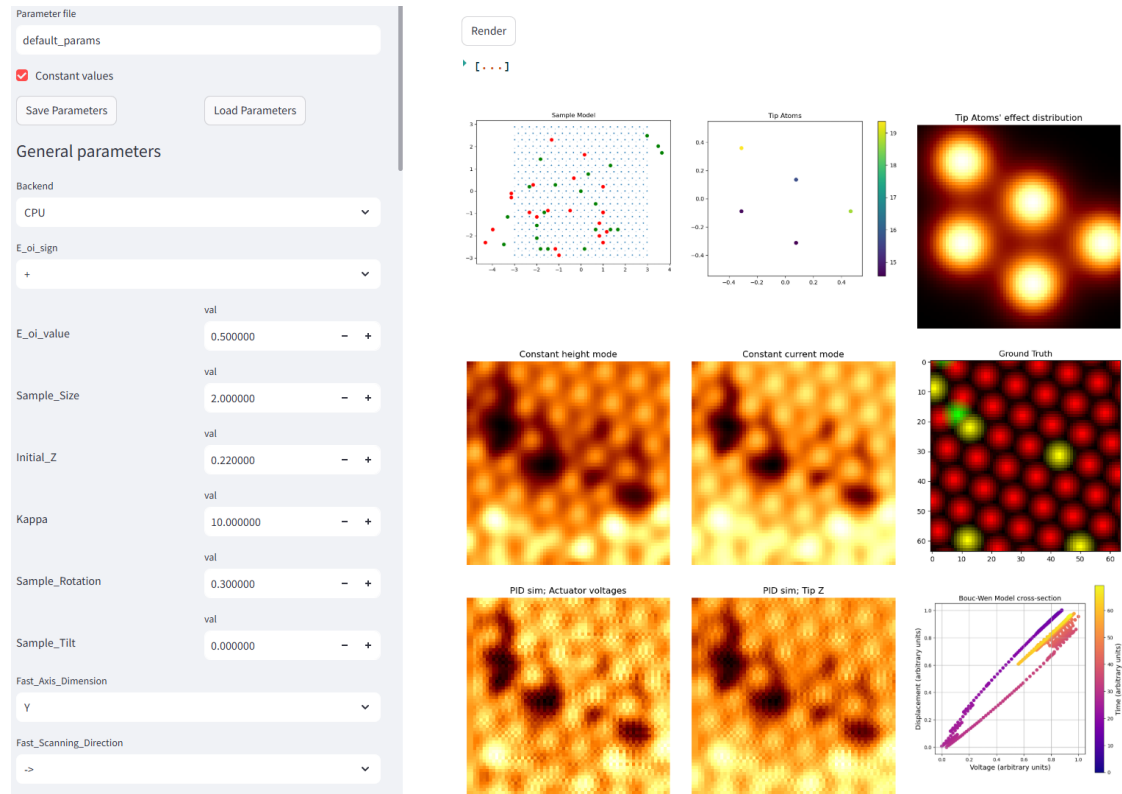
Figure 2.4: Graphical User Interface for parameter selection.
