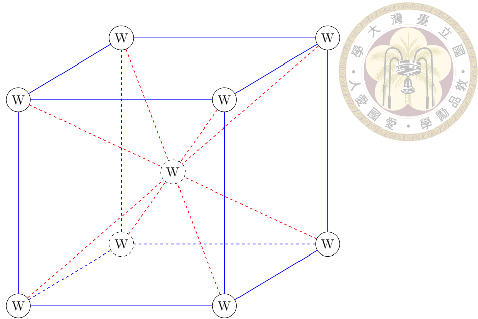
Figure 3.3: Tungsten lattice.
