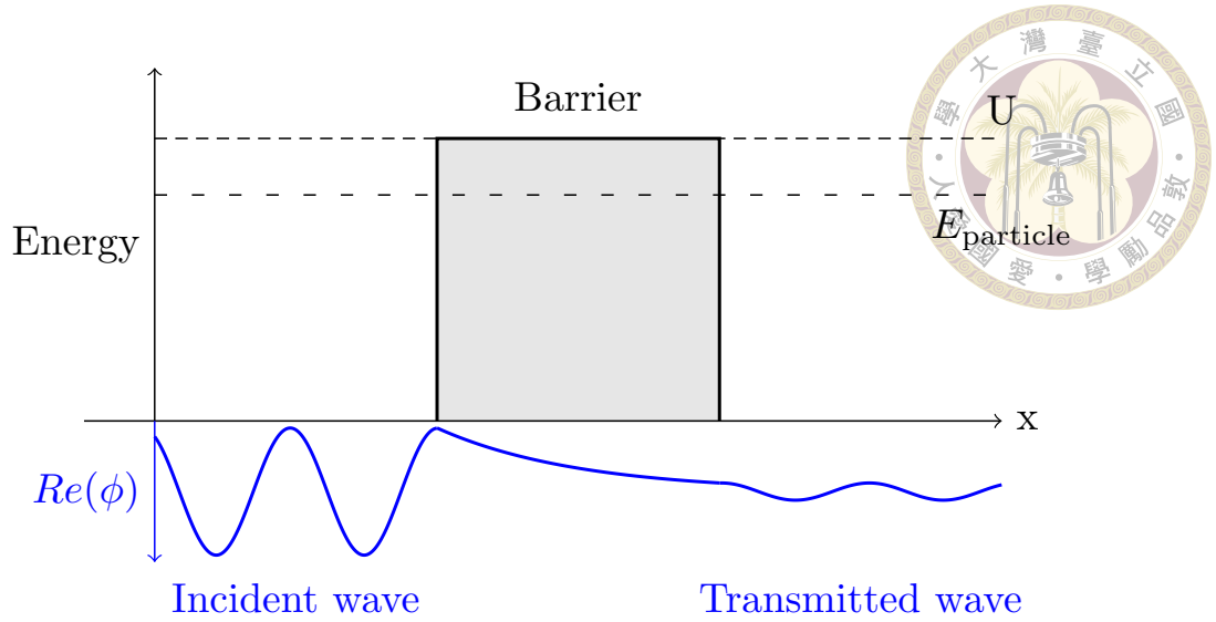
Figure 1.1: Illustration of an exponential decay through a potential barrier.
