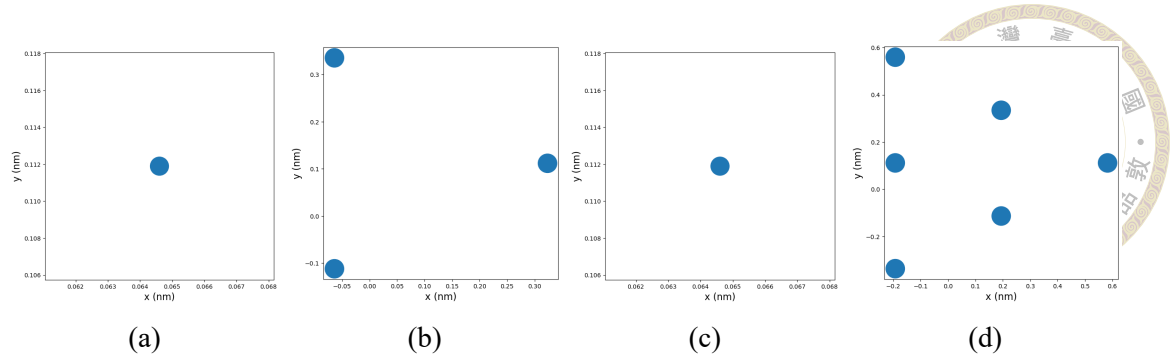
Figure 3.7: Atom positions in the 4 layers modelling the tip's apex.
