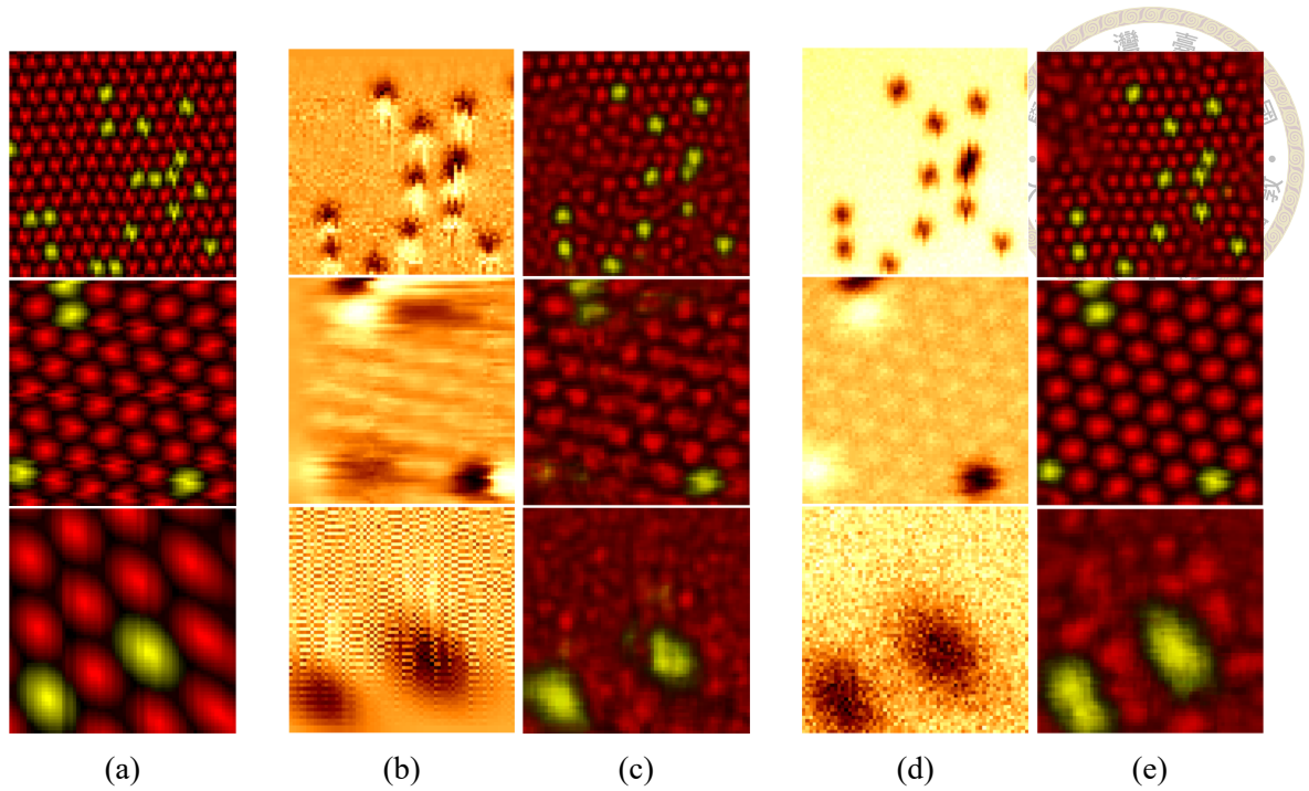
Figure 3.15: Validation of UNet defect localization model on synthetic data. (a) Ground Truth. (b) Main U-Net input. (c) Main U-Net output. (d) Control U-Net input. (e) Control U-Net output.
