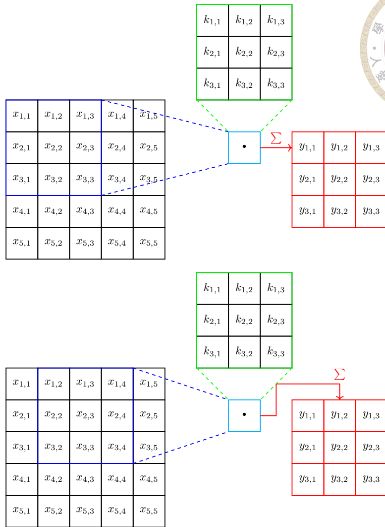
Figure 1.8: Illustration of a convolution with a stride of one pixel.
