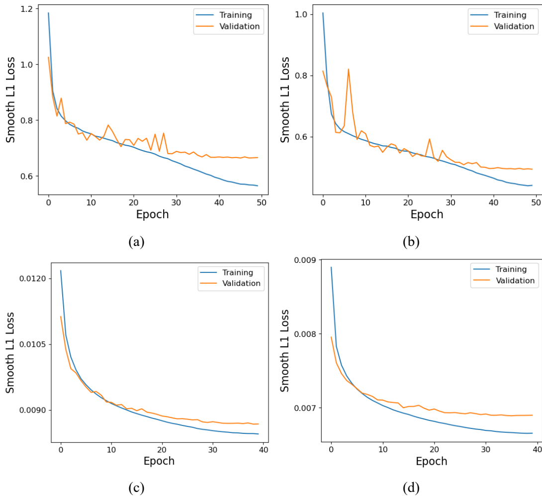
Figure 3.14: Loss over epochs. (a) Main ResNet, (b) Control ResNet, (c) Main U-Net, (d) Control U-Net.
