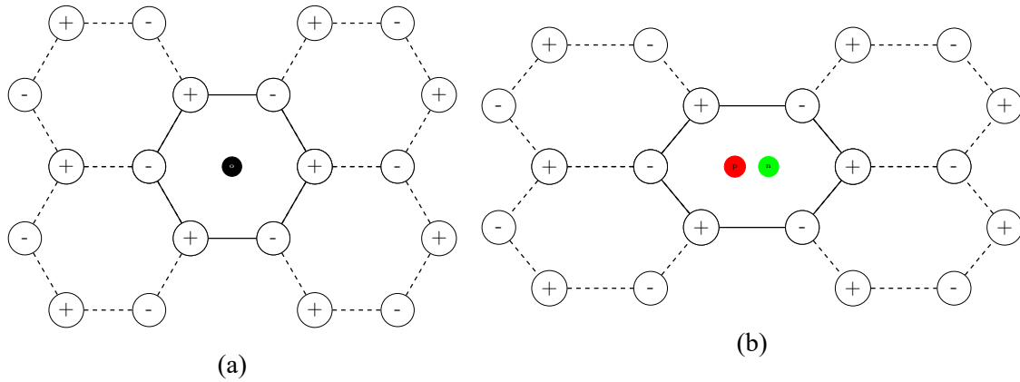
Figure 1.3: Illustration of the piezoelectric effect. (a) Unstrained crystal, charges cancel out. (b) Strained crystal, generating a polarization.
