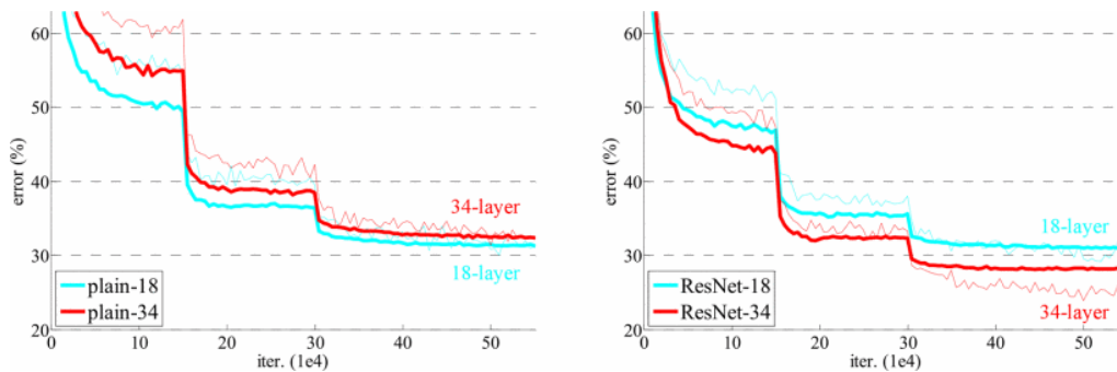
Figure 1.11: Comparison of training errors for models of different depths. The left figure shows that, without residual connections, error increases with depth. In contrast, the right figure shows that models containing residual connections achieve lower training error with greater depth. Taken from [1] © 2016 IEEE.
