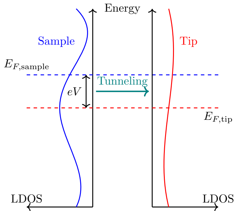
Figure 1.2: Illustration of the quantum tunneling dependence on DOS.
