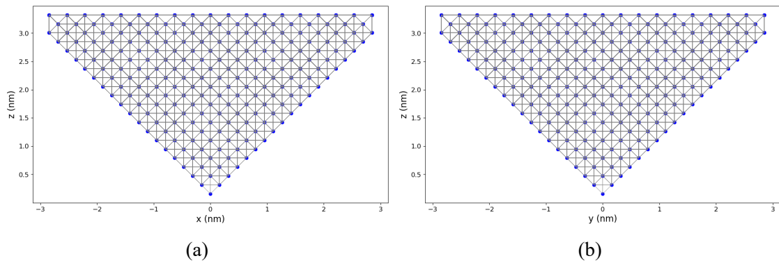
Figure 3.8: Model of the (001) tip. (a) Side view through the y axis. (b) Side view through the x axis.
