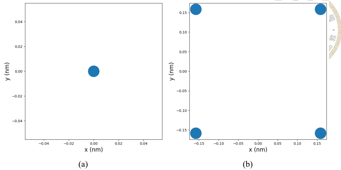
Figure 3.9: Atom positions in the 2 layers modelling the tip apex.
