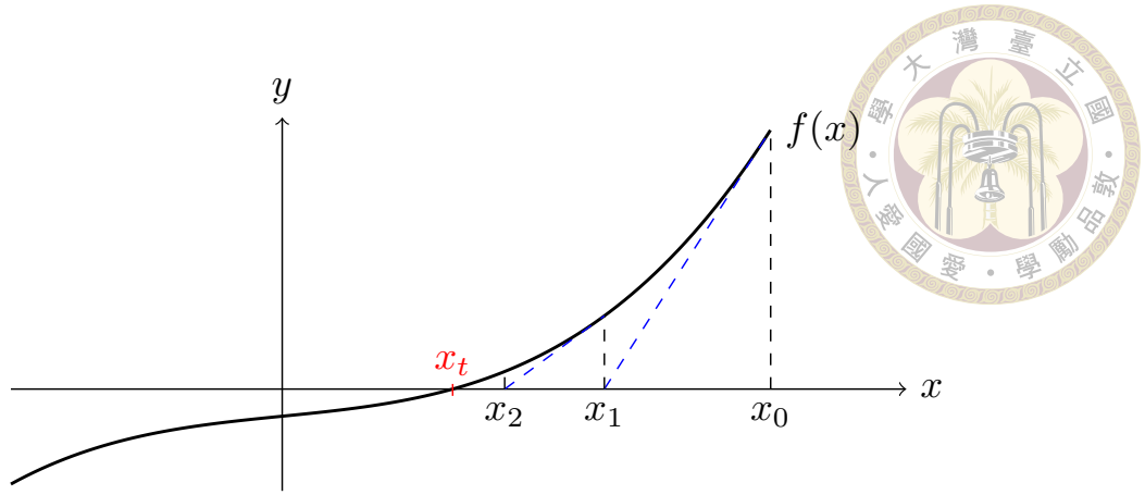
Figure 1.12: Illustration of the Newton's method. Iterations x_0, x_1, x_2 approach the root x_t .
