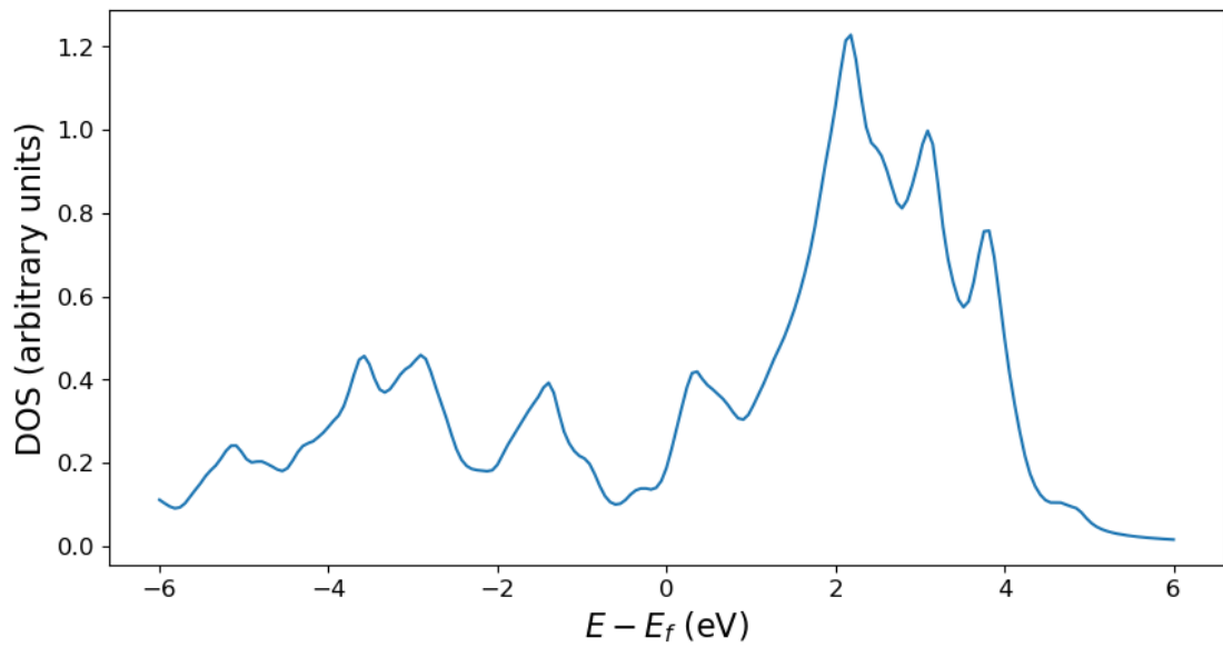
Figure 3.4: Simulated density of states for a tungsten atom in bulk.
