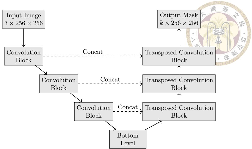
Figure 1.10: Illustration of the U-Net architecture.
