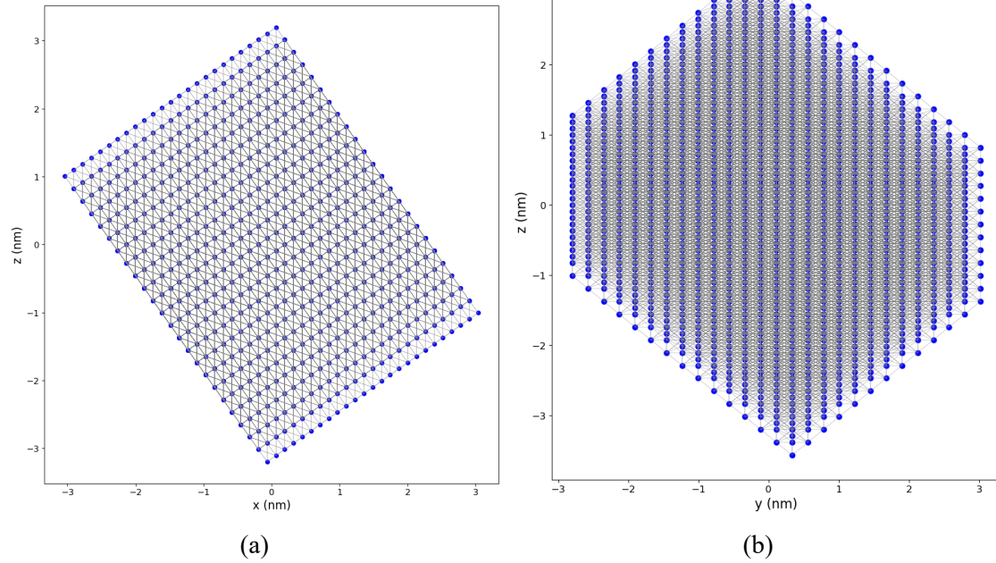
Figure 3.6: Model of the (111) tip. (a) x \times z side view. (b) y \times z side view.
