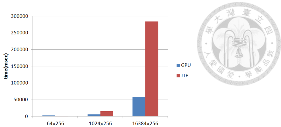
Figure 5.2: SC benchmark running in JTP and GPU modes
