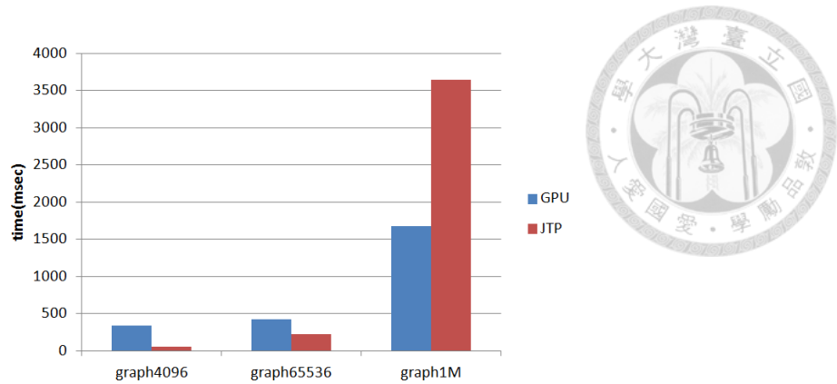
Figure 5.1: BFS benchmark run in JTP and GPU modes
