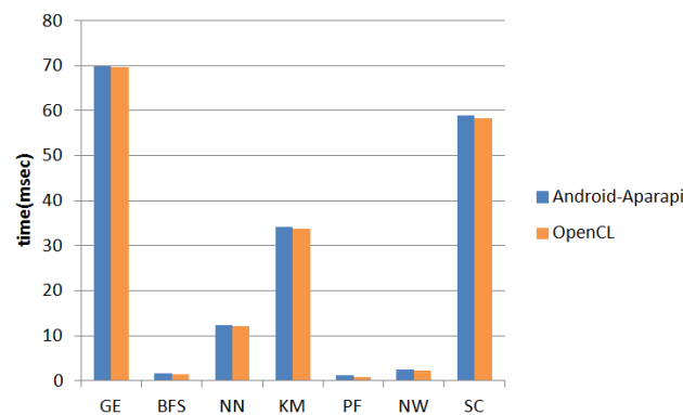
Figure 5.4: Large problem size of each benchmark
