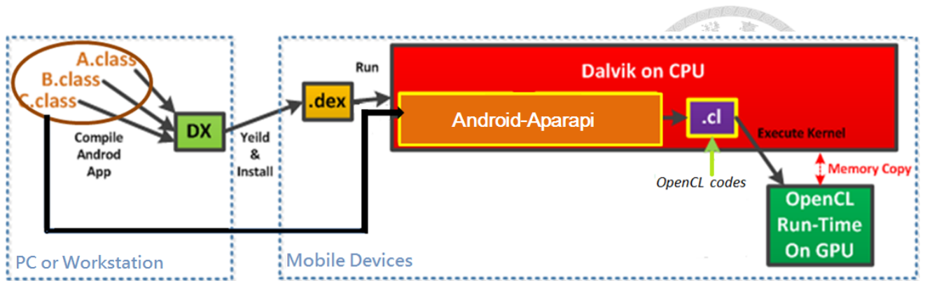
Figure 3.1: Architecture of Android-Aparapi on Android systems. On the PC or workstation, we package all the class format files which contains kernel class of Android-Aparapi. These files are passed to Android-Aparapi on Mobile devices. Android-Aparapi parse these files to generate OpenCL kernels, which are executed on the mobile GPU at run time.
