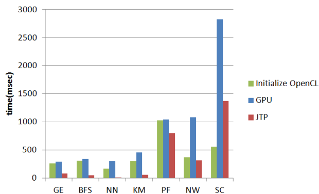
Figure 5.3: Small problem size of each benchmark
