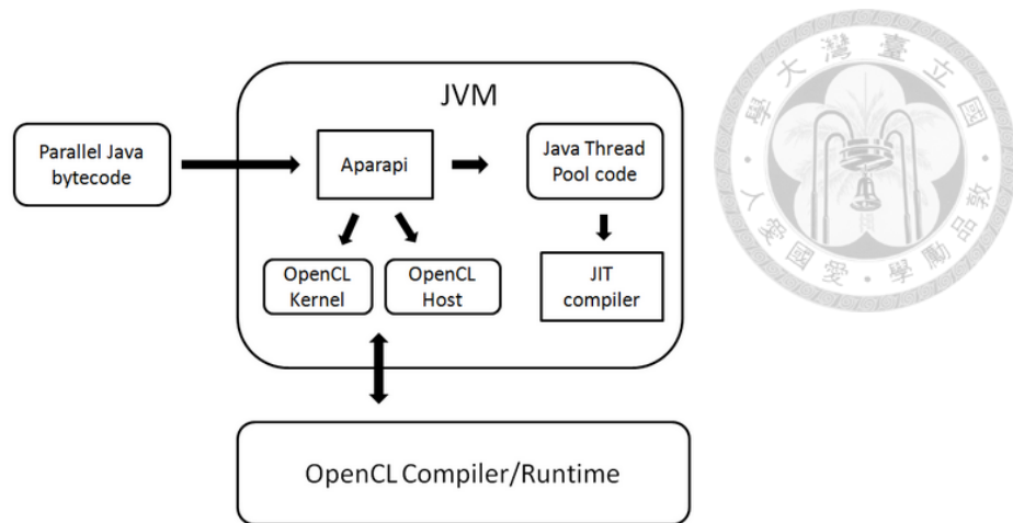
Figure 2.2: The flow of Aparapi: Convert Java bytecode to OpenCL host and kernel codes or to codes that uses Java thread pool
