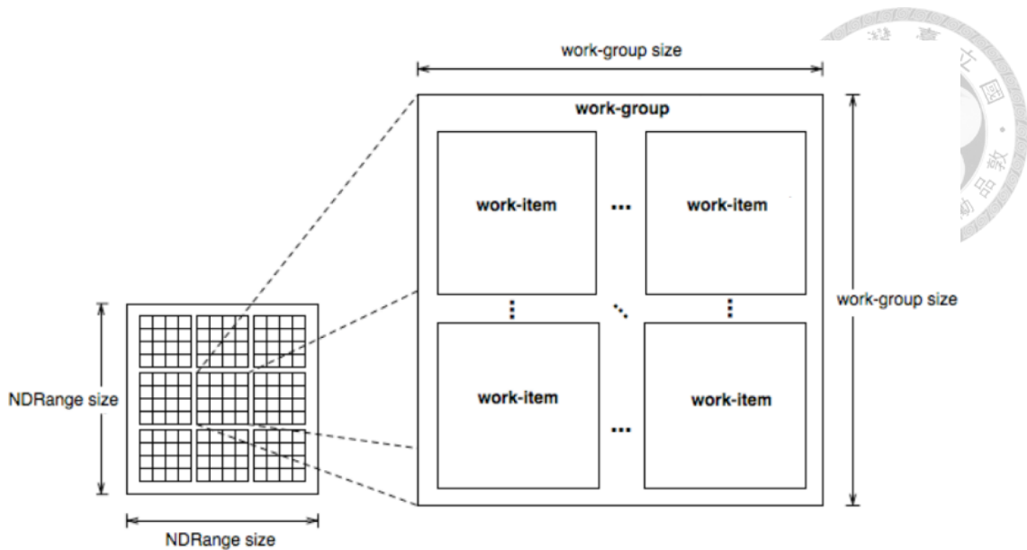
Figure 2.1: The structure of OpenCL work-items and work-groups
