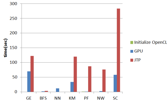
Figure 5.4: Large problem size of each benchmark
