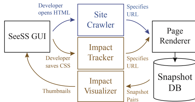
Figure 3.1: The 1st iteration SeeSS system architecture and data flow.
