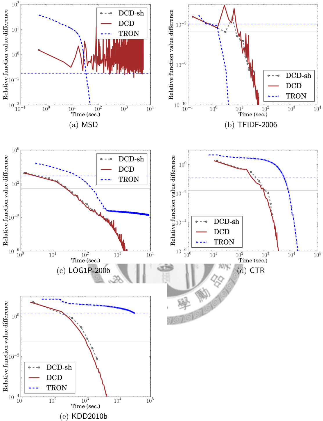
Figure 4.2: Relative differences to the optimal primal function value of L2-loss SVR using C = 1 and \epsilon = 0.1 . Original data without normalization are used. The dotted and solid horizontal lines respectively indicate the function values of TRON using \epsilon_s = 0.001 in (3.2) and DCD using \epsilon_s = 0.1 in (3.19).
