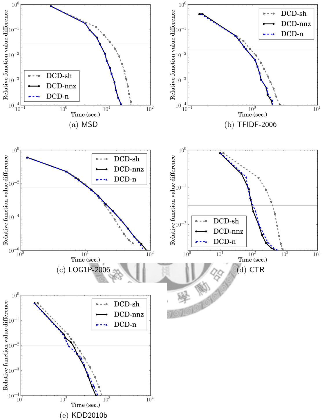
Figure 4.8: A comparison of three shrinking settings. L1-SVR with C = 1 and \epsilon = 0.1 is applied on normalized data. We show the relative difference to the dual optimal function values and training time (in seconds).
