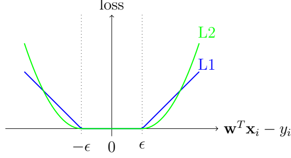
Figure 2.1: L1-loss and L2-loss functions.
