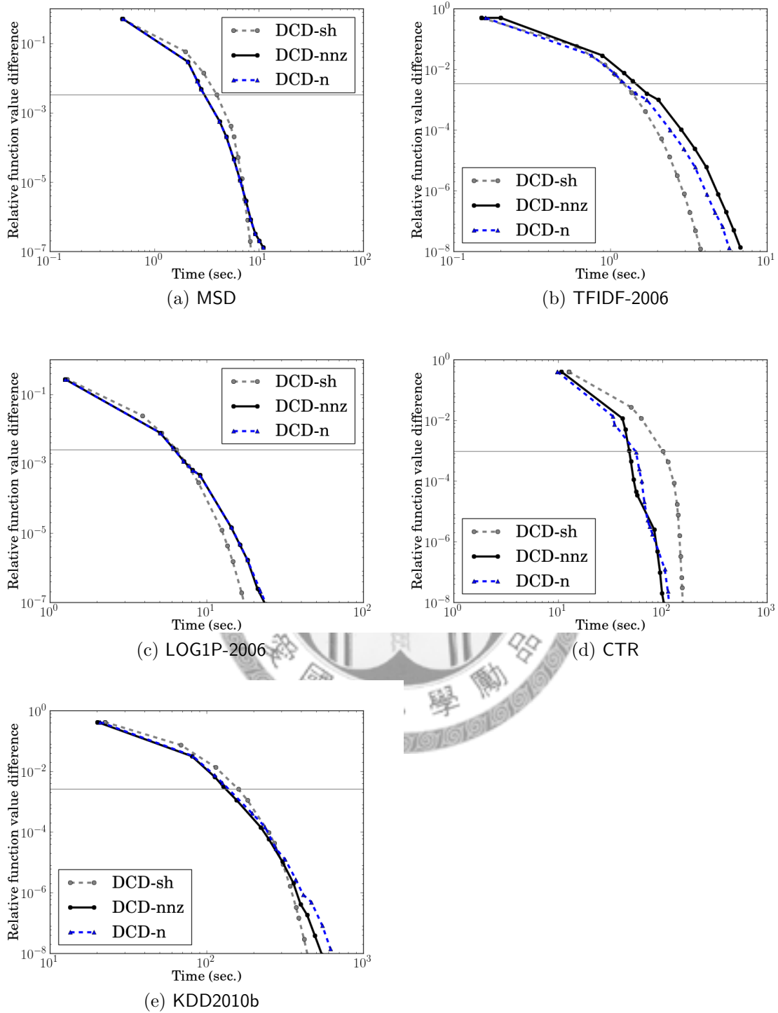
Figure 4.9: A comparison of three shrinking settings. L2-SVR is used. Other settings are the same as those in Figure 4.8.
