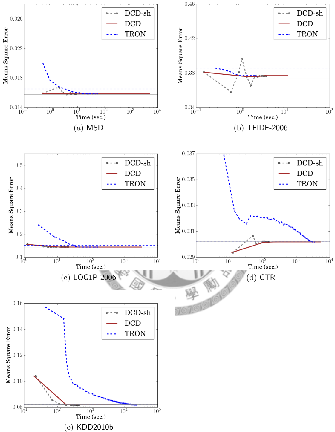
Figure 4.6: MSE of L2-loss SVR. Settings are the same as those in Figure 4.5.
