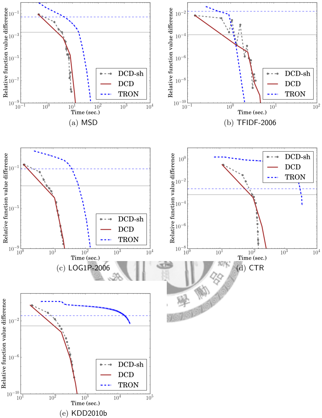
Figure 4.5: Relative differences to the optimal primal function value of L2-loss SVR using C = 1 and \epsilon = 0.1 . Data instances are normalized to unit vectors. The dotted and solid horizontal lines respectively indicate the function values of TRON using \epsilon_s = 0.001 in (3.2) and DCD using \epsilon_s = 0.1 in (3.19).
