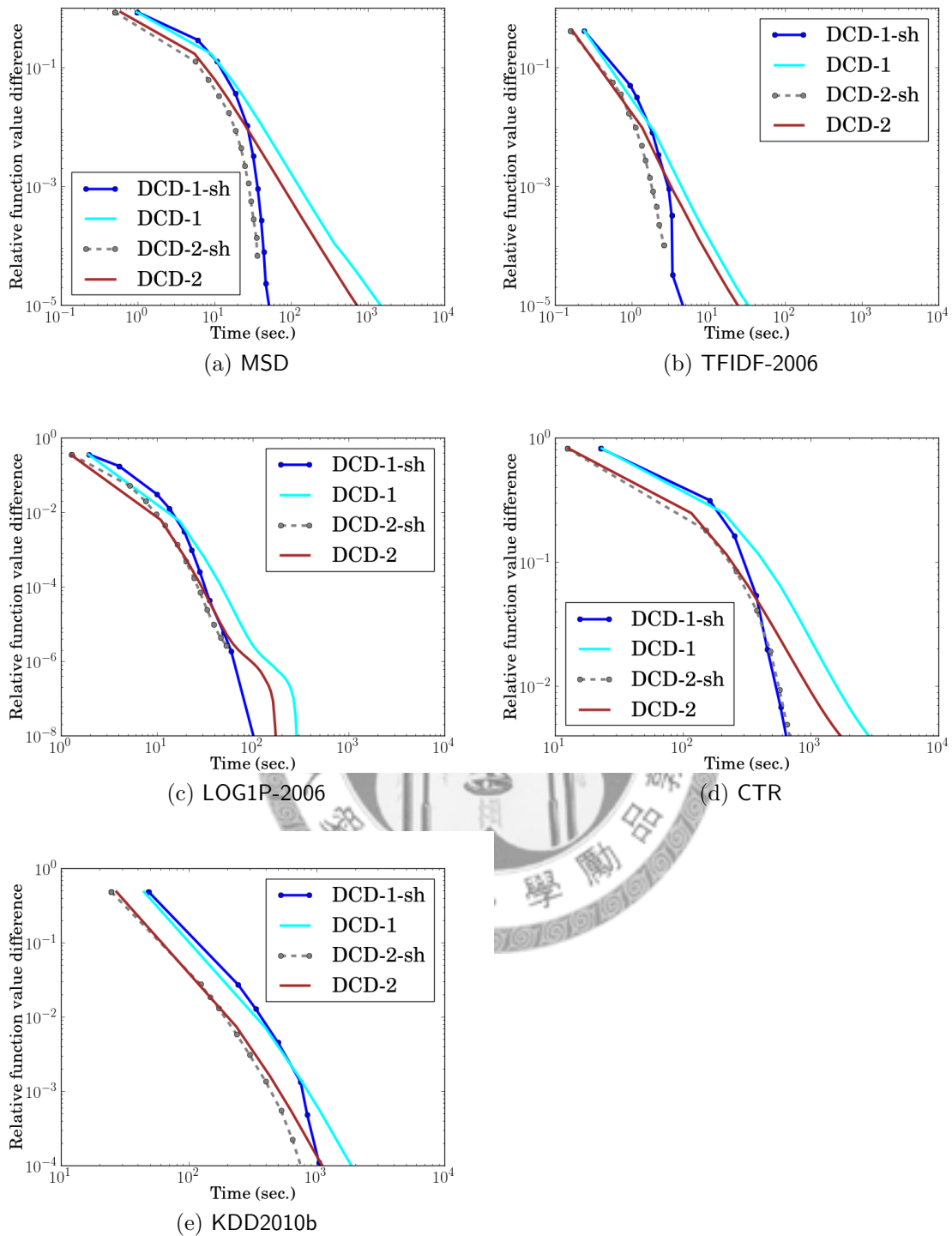
Figure 4.1: Relative difference to the dual optimal function values of L1-loss SVR using C = 1 and \epsilon = 0.1 . Data instances are normalized to unit vectors. DCD-1-sh and DCD-2-sh are DCD-1 and DCD-2 with shrinking, respectively. Both x -axis and y -axis are in log scale.
