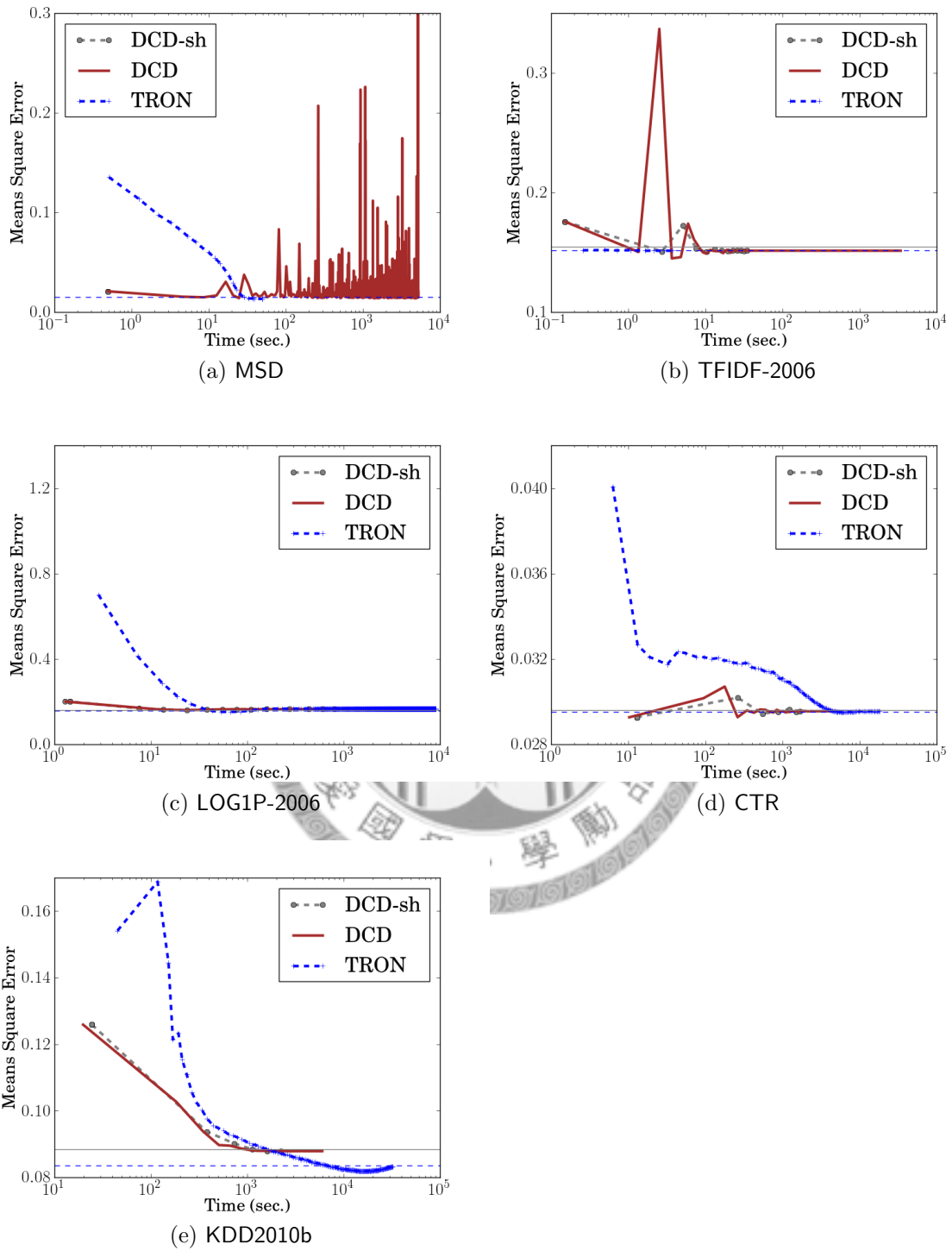
Figure 4.3: MSE of L2-loss SVR. Settings are the same as those in Figure 4.2.
