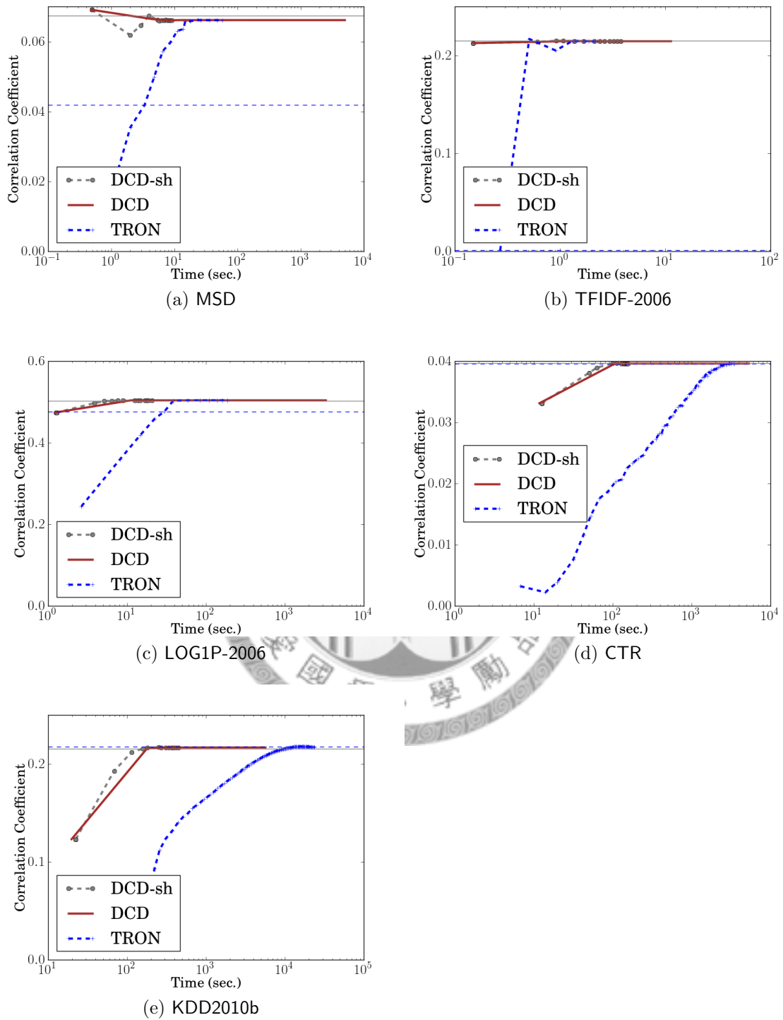
Figure 4.7: R^2 of L2-loss SVR. Settings are the same as those in Figure 4.5.
